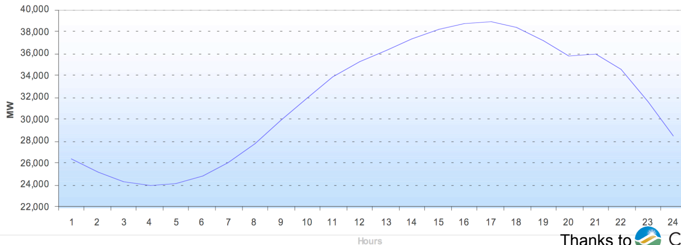
Total Wind -- Summer 2006
